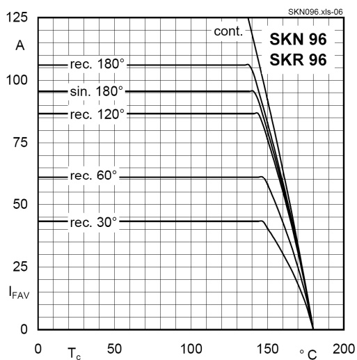
Fig. 2 Forward current vs. case temperature
