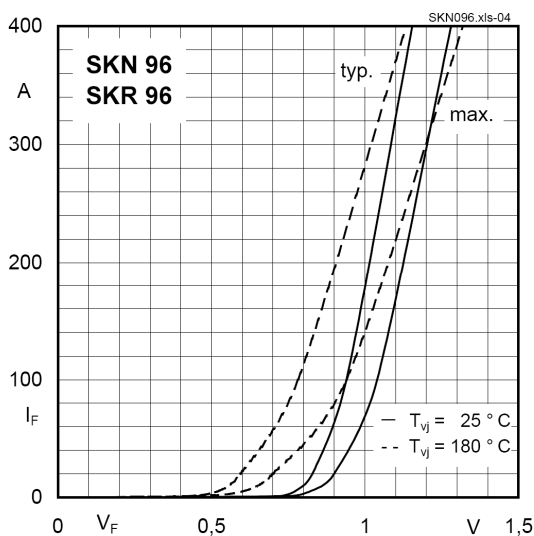
Fig. 5 Forward characteristics
