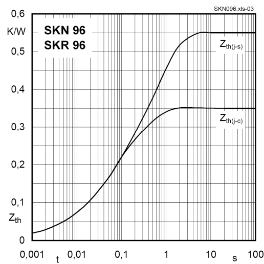
Fig. 4 Transient thermal impedance vs. time
