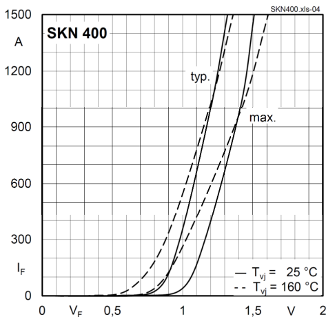
Fig. 5 Forward characteristics
