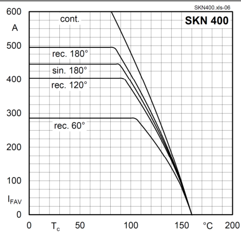
Fig. 2 Forward current vs. case temperature
