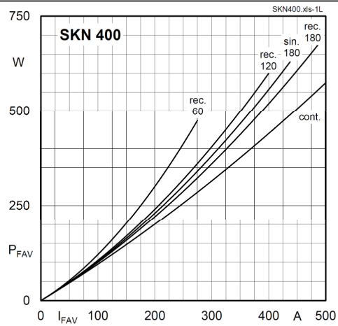
Fig. 1L Power dissipation vs. forward current
