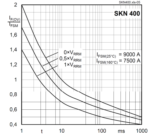
Fig. 6 Surge overload current vs. time
