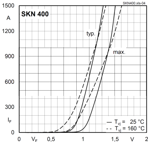
Fig. 5 Forward characteristics
