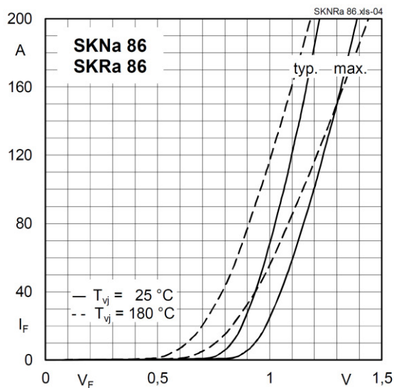
Fig. 5 Forward characteristics
