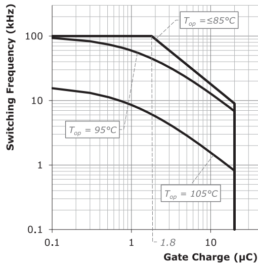
Fig. 1: Maximum Switching Frequency
