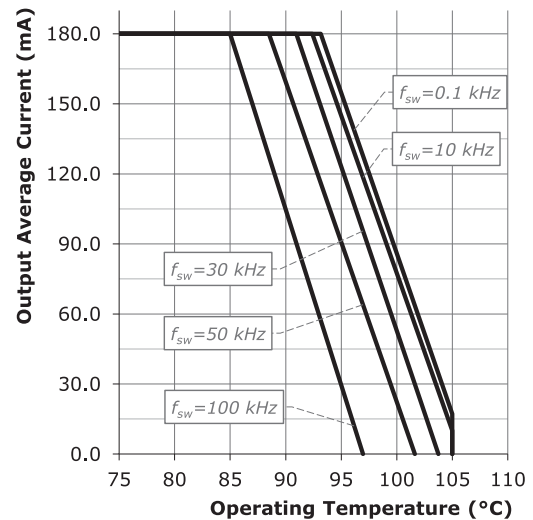
Fig. 2: Output Average Current
