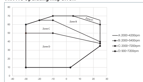
VRN752 Operating map SH 5K
