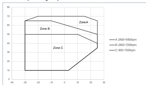
VRN226 Operating map SH 5K
