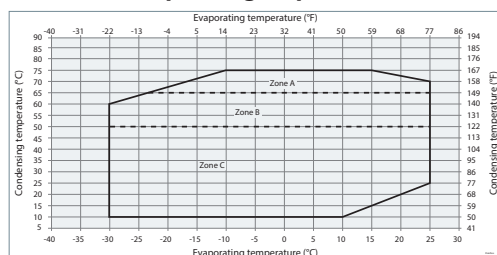
VRN418-548 Operating map SH 5K
