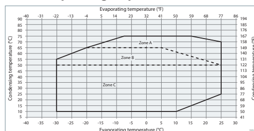
VRN752 Operating map SH 5K
