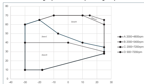
VRN307 with single phase drive Operating map SH 5K
