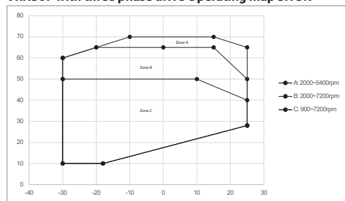
VRN548 Operating map SH 5K
