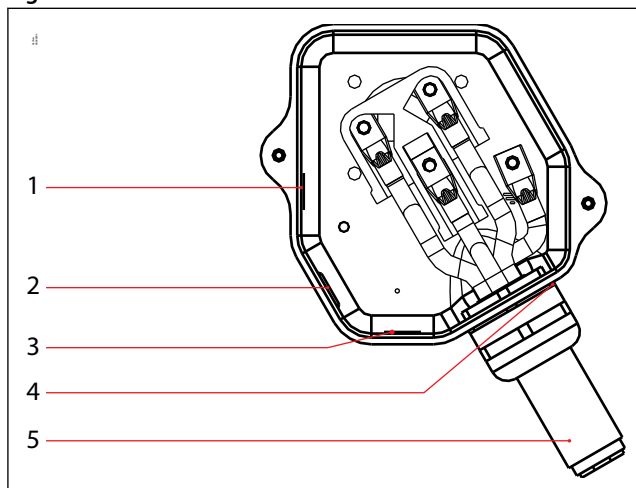
Figure 22: terminal box for VZF088/117-J
