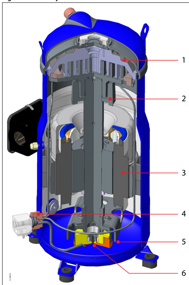
Figure 1: Cut Away VZF
