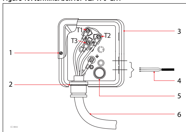
Figure 19: terminal box for VZF170-G/H
