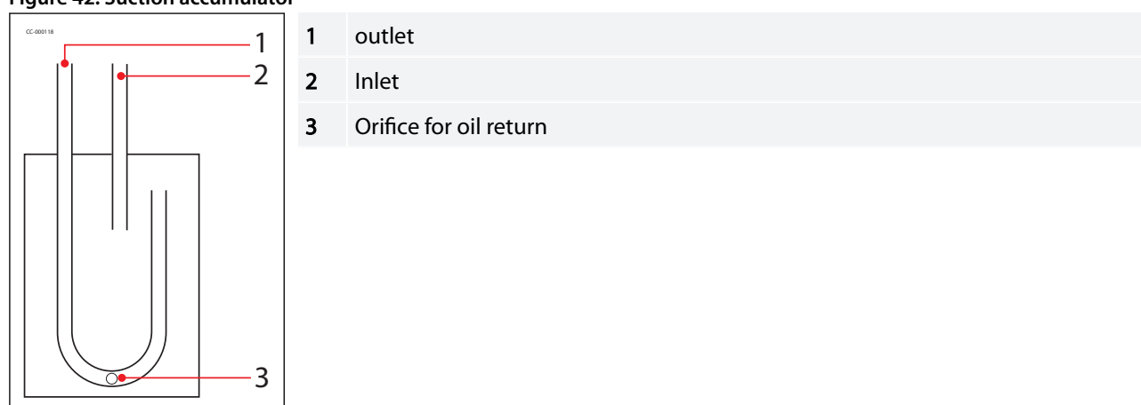
Figure 42: Suction accumulator
