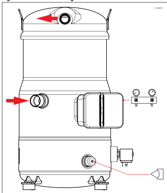
Figure 14: Outline drawing 2
