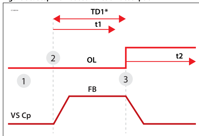
Figure 36: Step 1 Oil boost Function description
