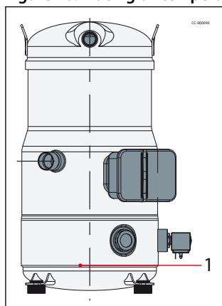
Figure 40: Placing oil temperature sensor
