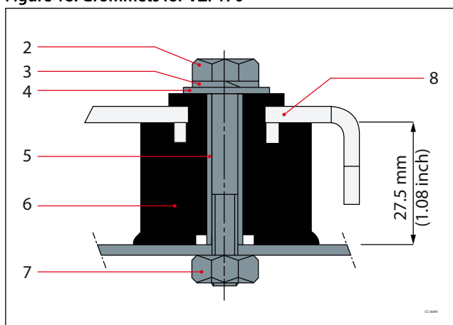
Figure 18: Grommets for VZF170
