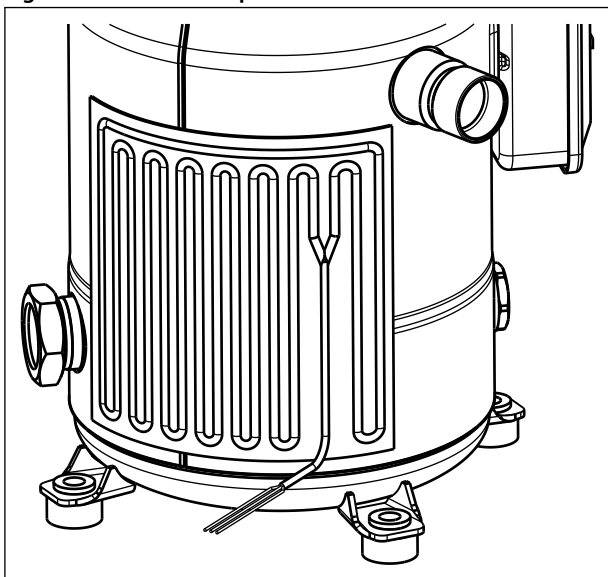
Figure 44: Surface sump heater for VZF088-117
