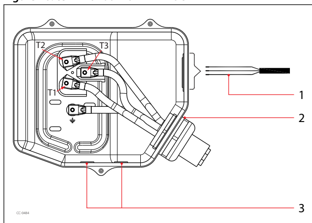
Figure 20: terminal box for VZF170-J
