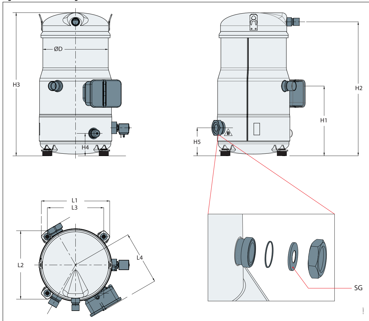
Figure 5: Outline drawing number 2
