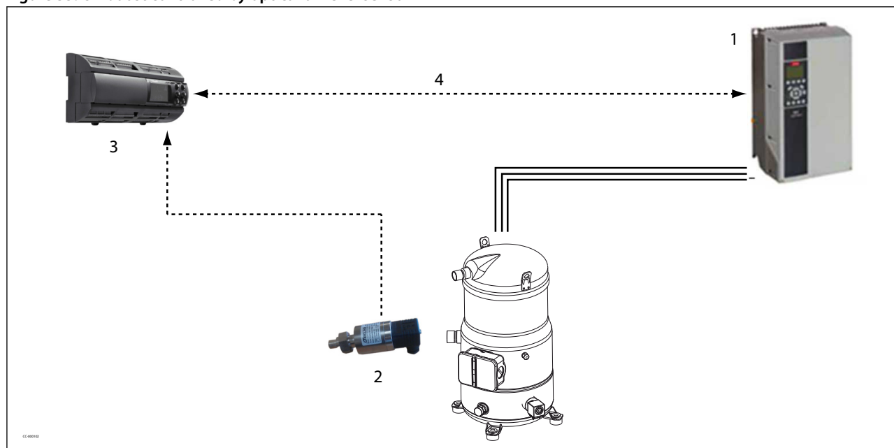
Figure 35: Oil boost controlled by optical oil level sensor
