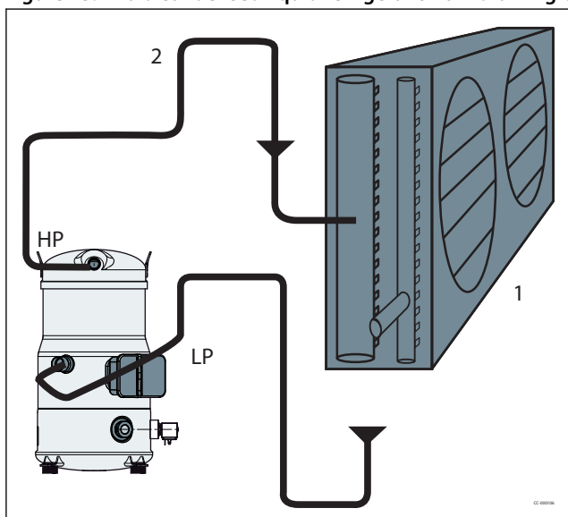
Figure 43: Avoid condensed liquid refrigerant from draining back
