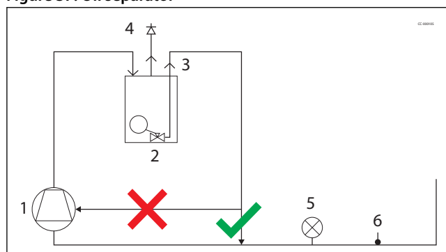
Figure 37: Oil separator
