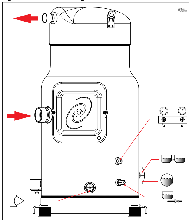
Figure 16: Outline drawing 4
