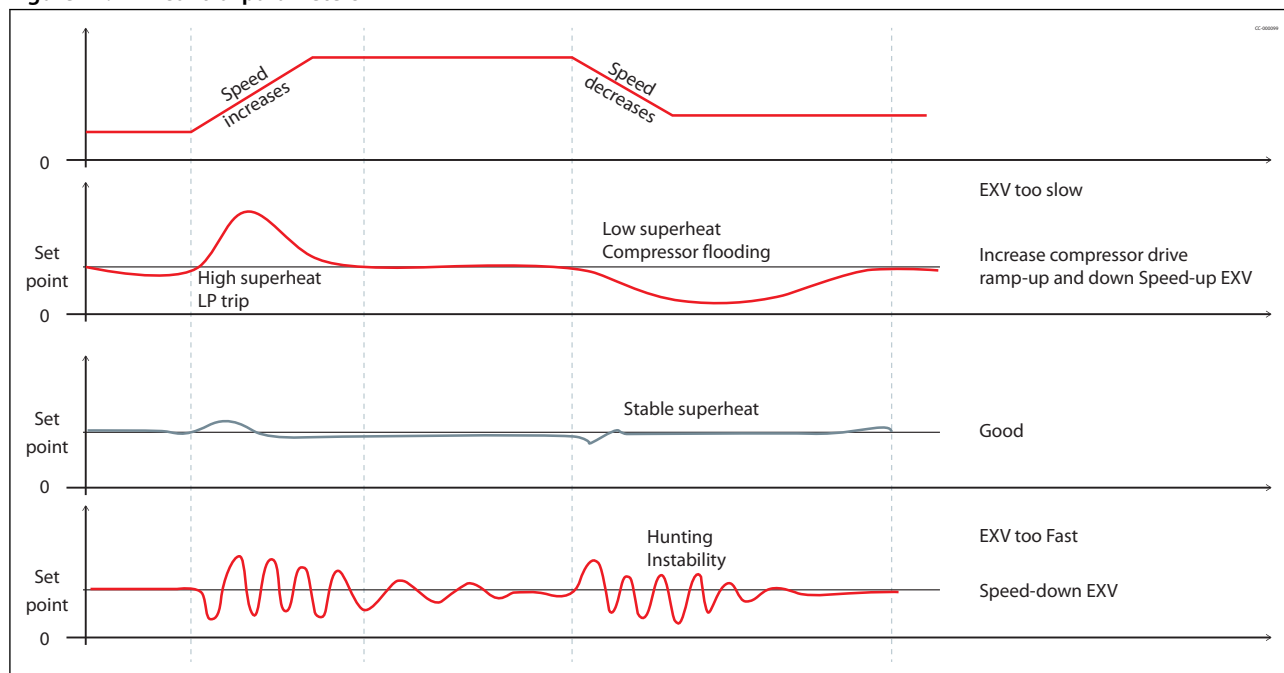
Figure 41: EXV control parameters
