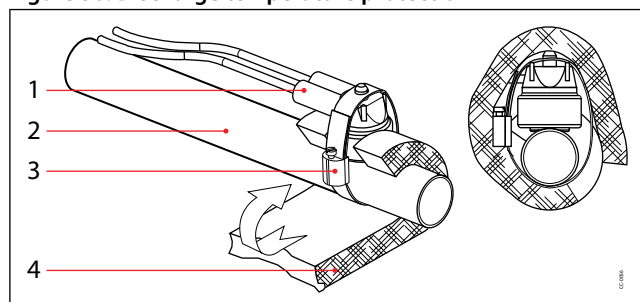
Figure 30: Discharge temperature protection
