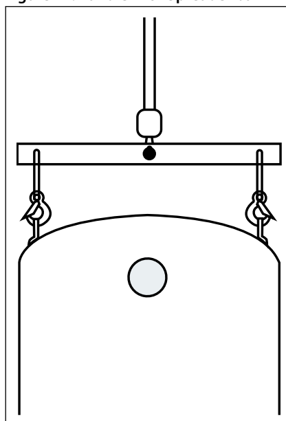
Figure 47: handle with Spreader bar
