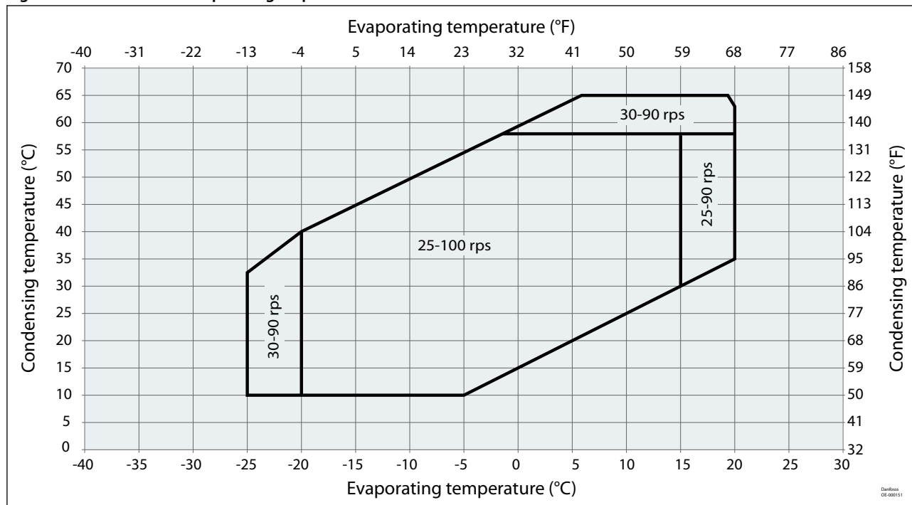
Figure 3: VZF088/117/170 Operating Map - R32
