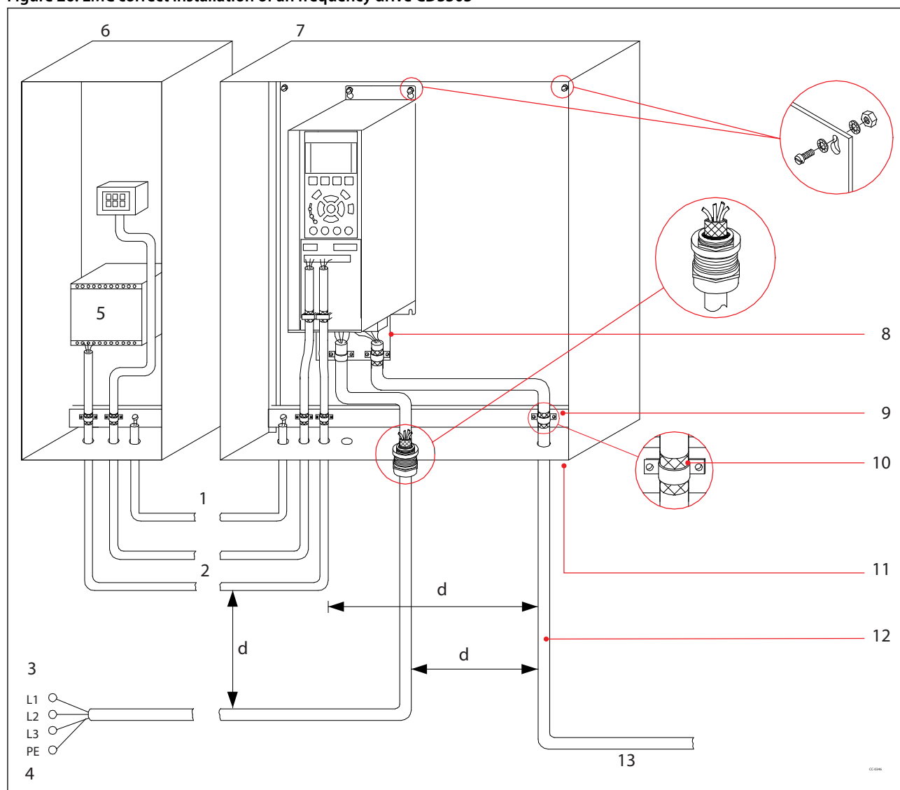
Figure 26: EMC correct installation of an frequency drive CDS303
