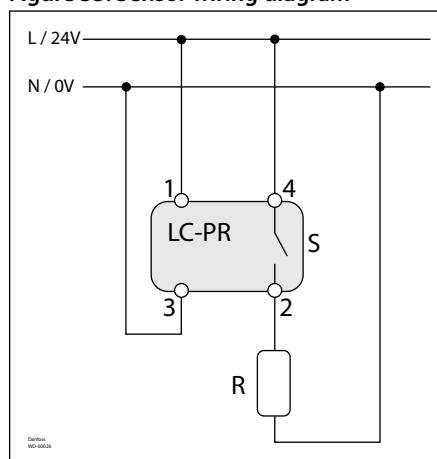
Figure 33: Sensor wiring diagram
