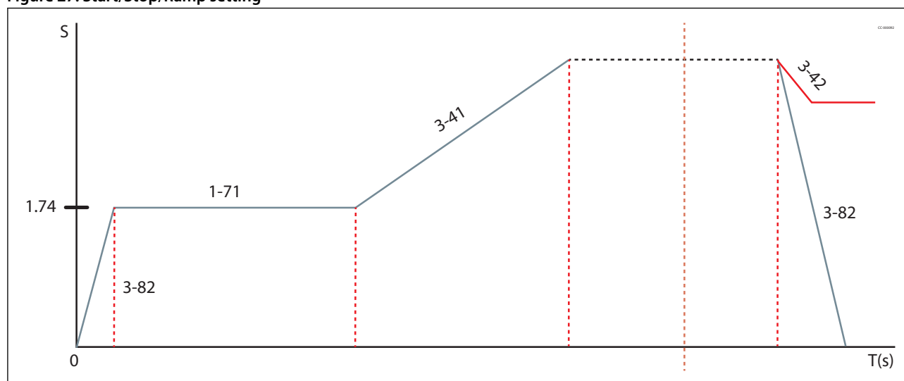
Figure 27: Start/Stop/Ramp setting
