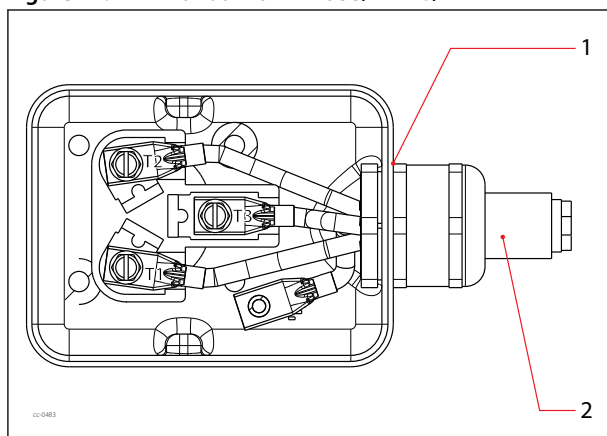
Figure 21: Terminal box for VZF088/117-G/H
