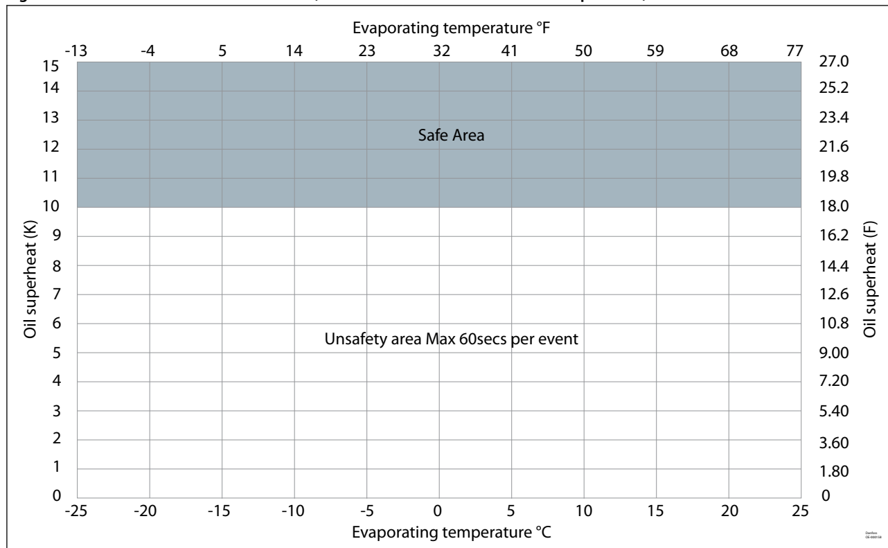
Figure 39: VZF170 R32 - Dilution chart (reference at 20°C / 68°F ambient temperature)
