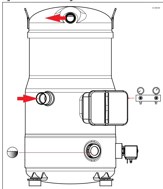
Figure 13: Outline drawing 1
