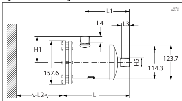
Figure 8: DCRE housing
