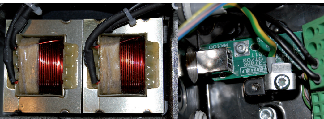
Built-in DC coils to limit harmonic distortion
