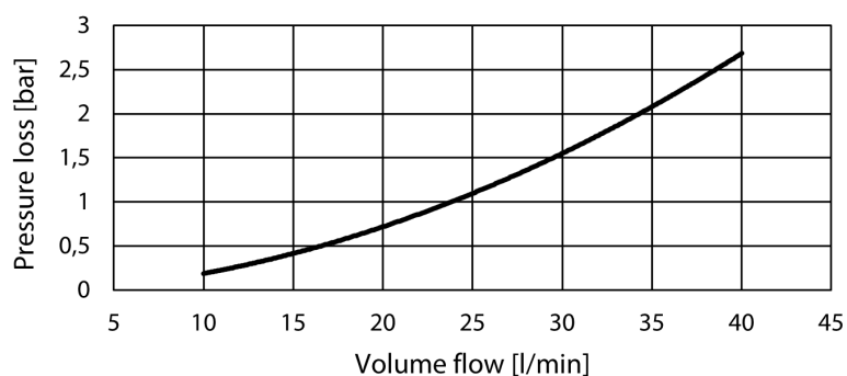
Picture 1 Pressure loss vs coolant flow (+25°C coolant)
