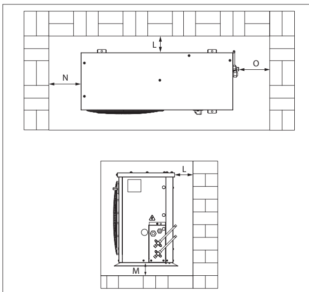
Picture 1 : Minimum mounting distances
