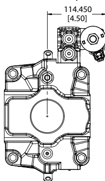
Radial Endcap Counterclockwise
