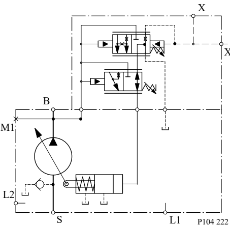
Schematic
