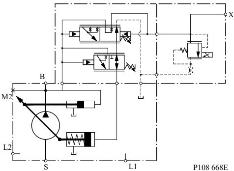
Schematic
