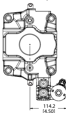
Axial Endcap Clockwise
