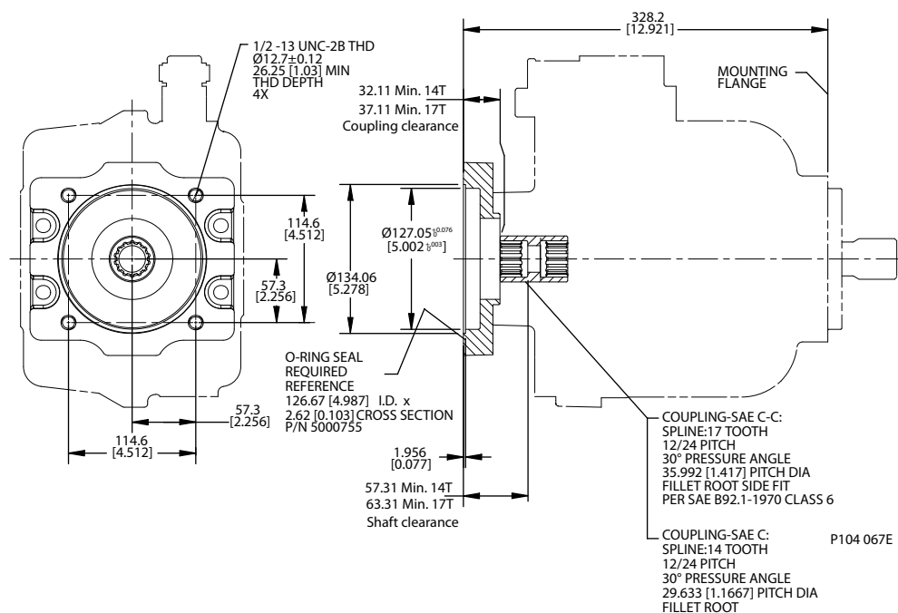
SAE-C Dimensions
