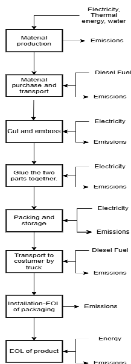
Figure 5: Process flow diagram
