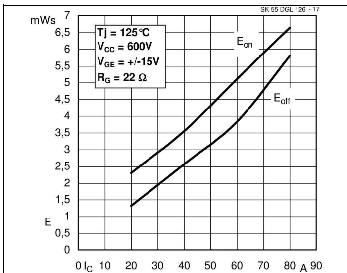
Fig. 17 Turn-on/off energy=f(Ic)
