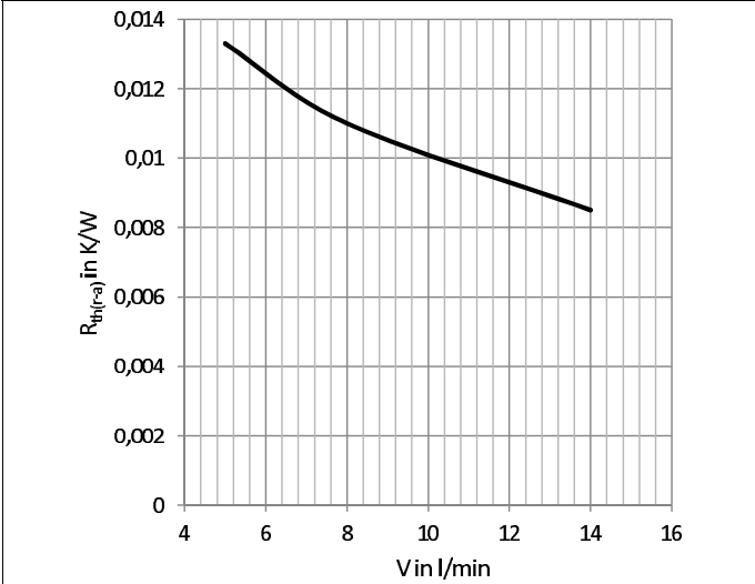
Fig. 9: Thermal resistance R_{th(r-a)} versus flow rate V
