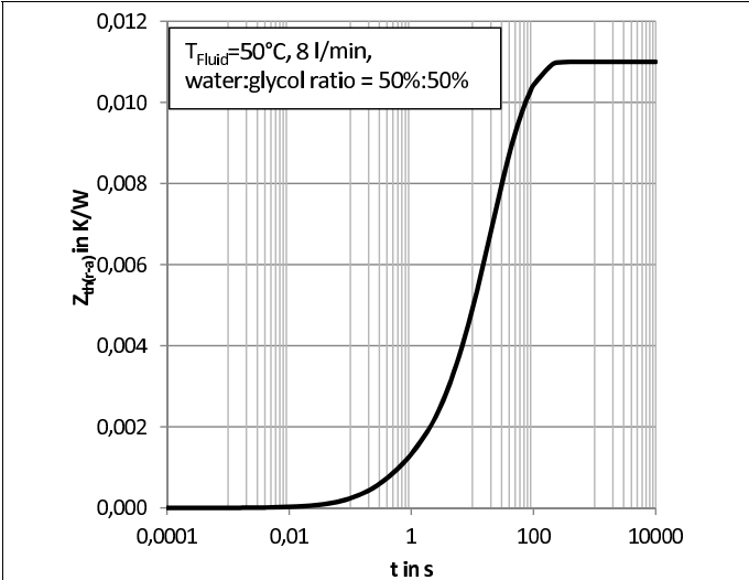
Fig. 7: Transient thermal impedance Z_{th(r-a)}
