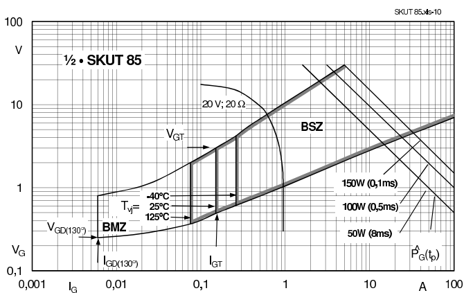
Fig. 10: Gate trigger characteristic
