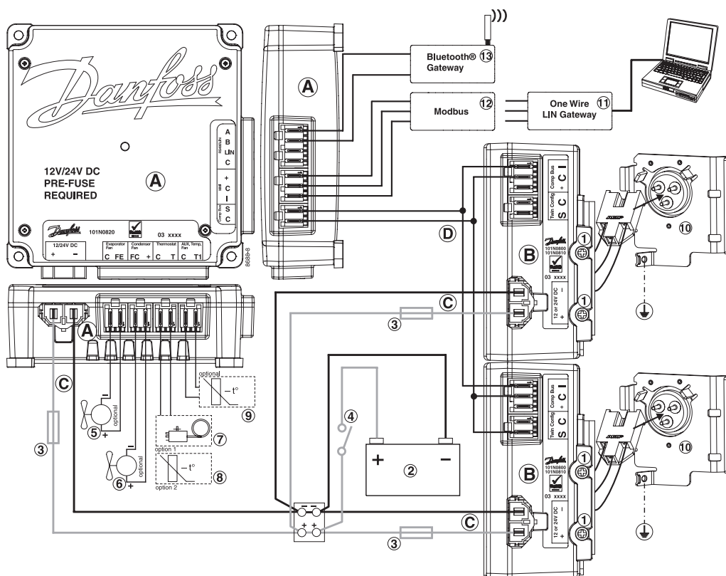
Wiring diagram
