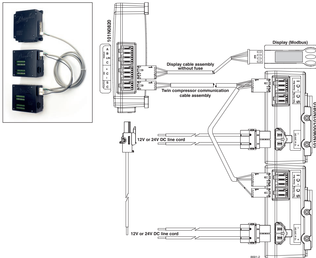
Wiring diagram
