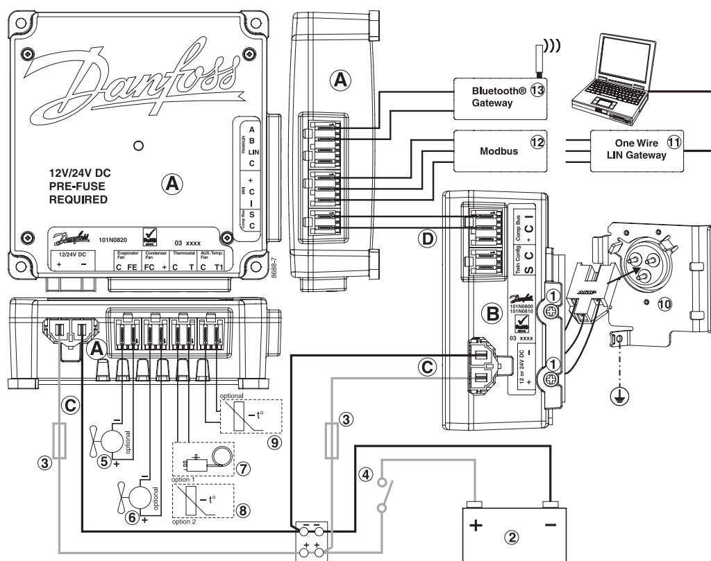
Wiring diagram
