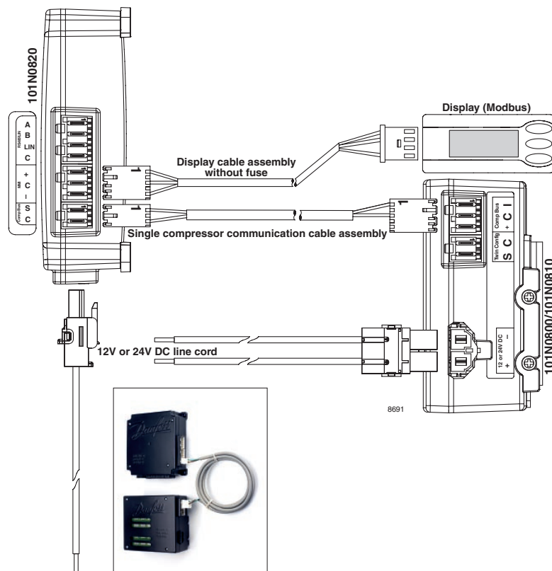
Wiring diagram
