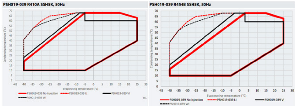
Updated envelope of PSH039 50Hz
