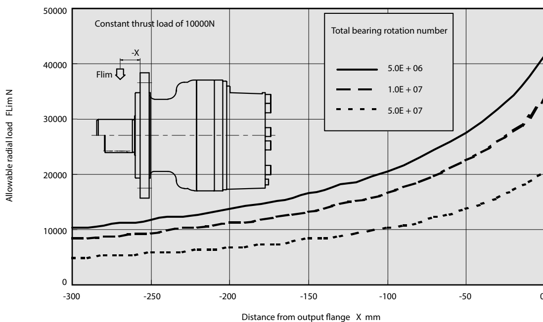
Fig.14 DCM0280 allowable radial load for the front flange type
