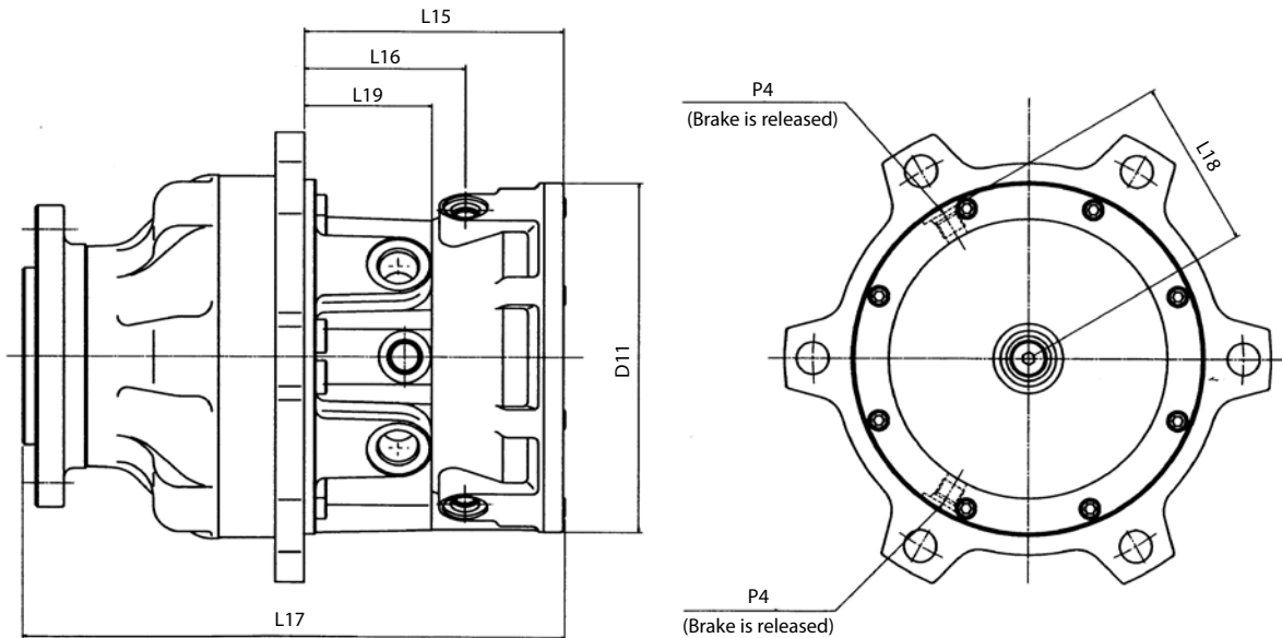
Fig.20 Brake dimensions
