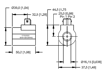
ASD Amp SuperSeal 1.5/MetriPak 150 Type 1 w/diode
