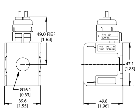
FLDB Lead wires w/diode
