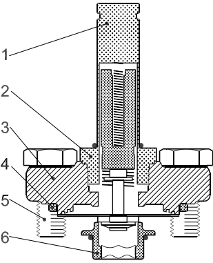
Figure: ICFE 20L solenoid valve module
