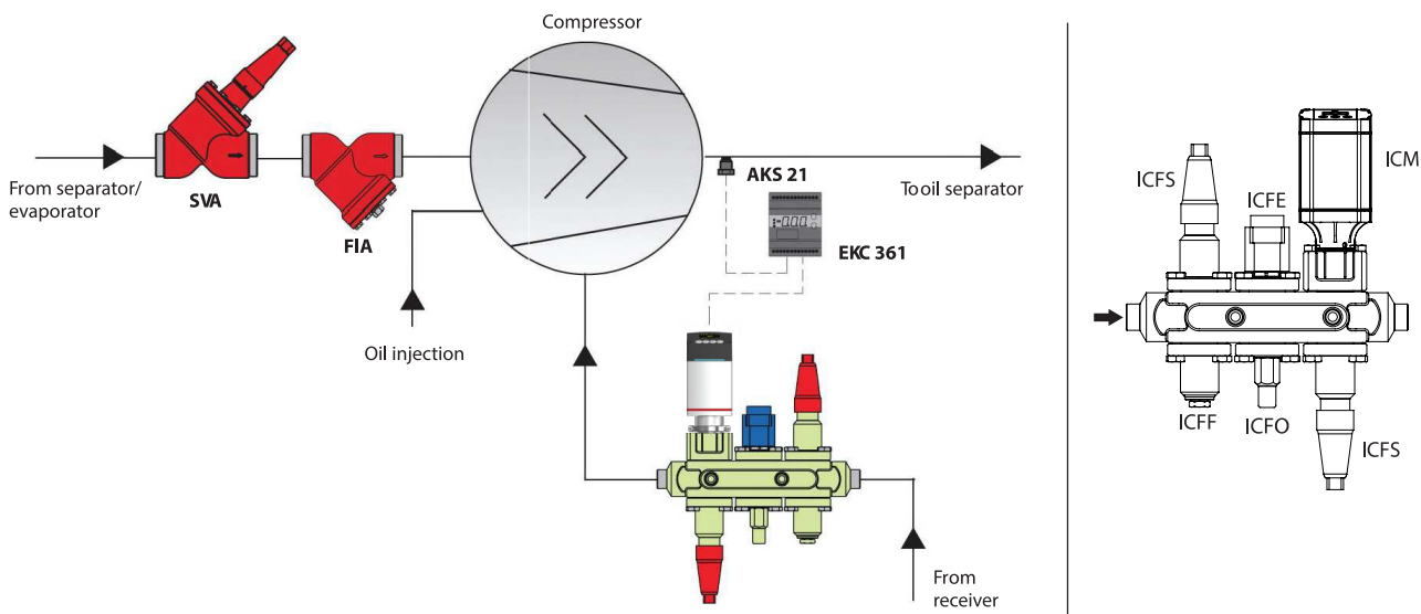
Figure: Valve combination for compressor
