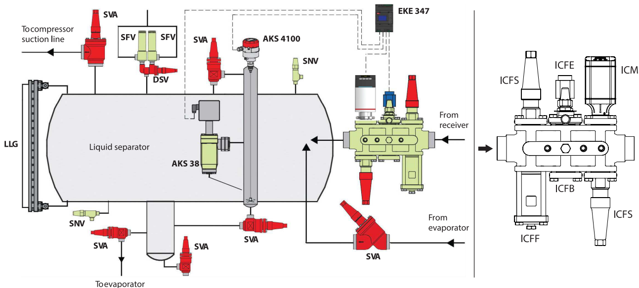
Figure: Valve combination for liquid injection
