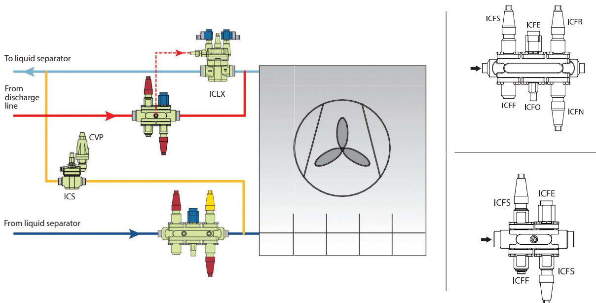
Figure: Liquid feed line / Hot gas defrost line
