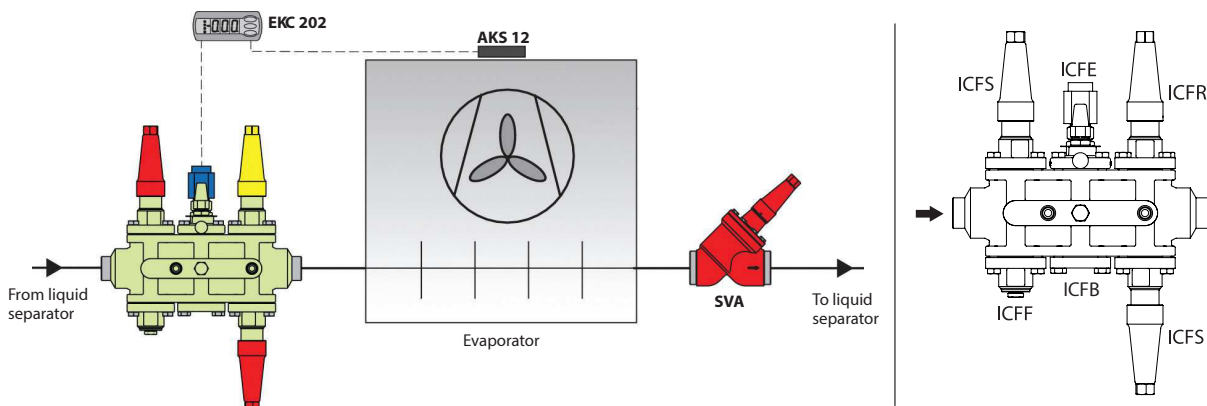
Figure: ICF configurations
