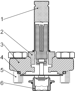
Figure: ICFE 20 solenoid valve module
