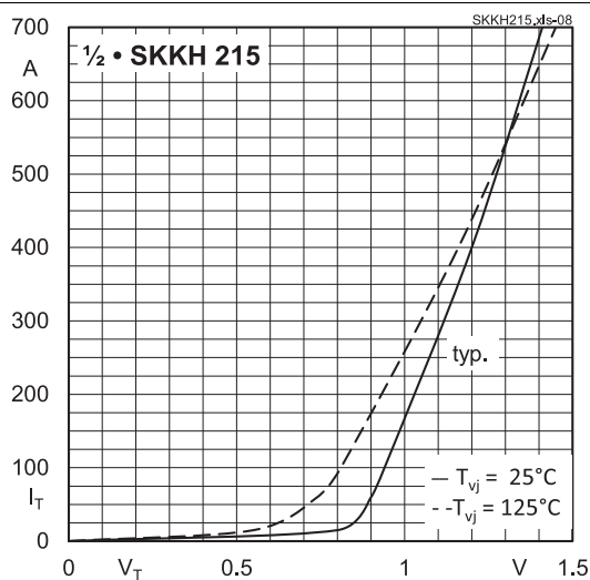
Fig. 7: On-state characteristics (chipelevel)
