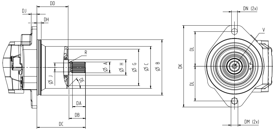
Cartridge flange dimensions, mm [in]
