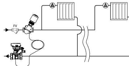
Fig. : The impulse tube must be flushed through before installation.
