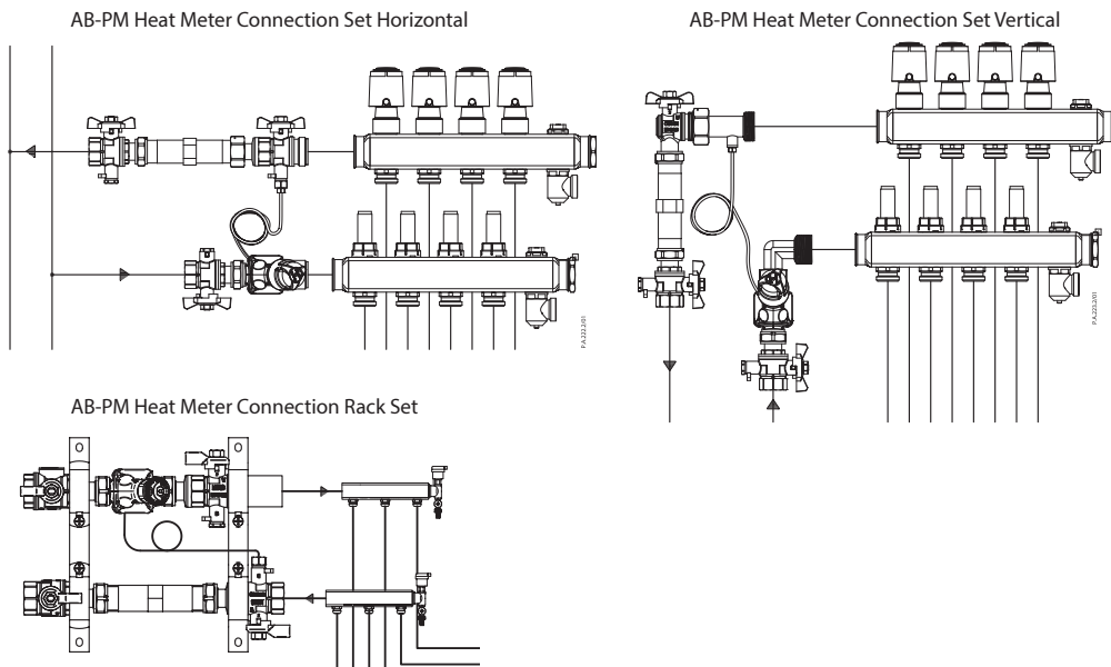
Fig.: AB-PM in manifold for floor heating system
