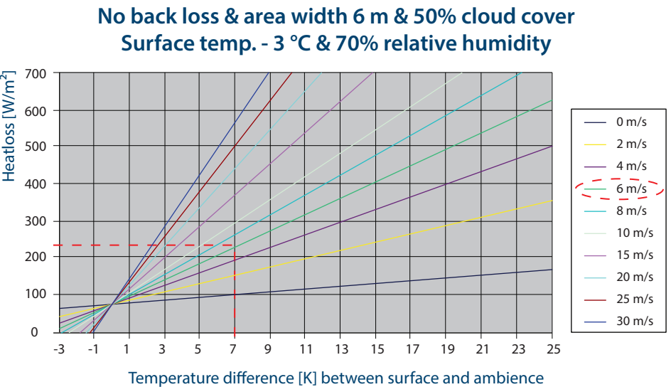
Fig. 2. Wind and temperature dependent heat loss
