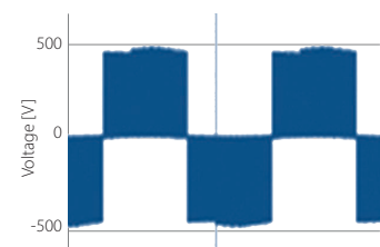
Conventional 2-level ULHD
