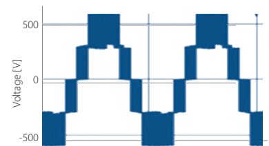
3-level iC7-HVACR ULH
