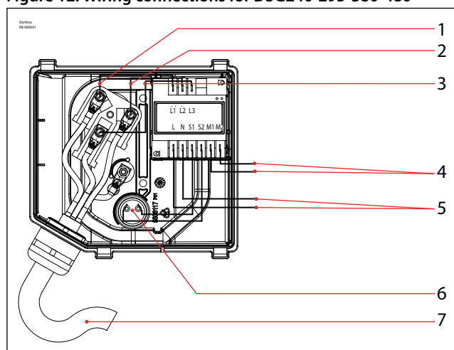
Figure 12: Wiring connections for DSG240-295-380-480
