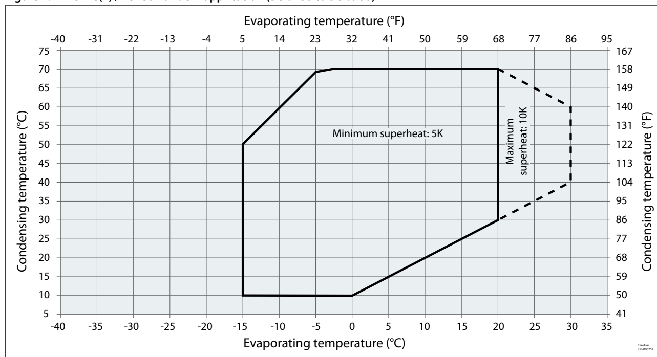
Figure 2: R1234ze(E) / R515B Tandem application (DSG480 to DSG960)
