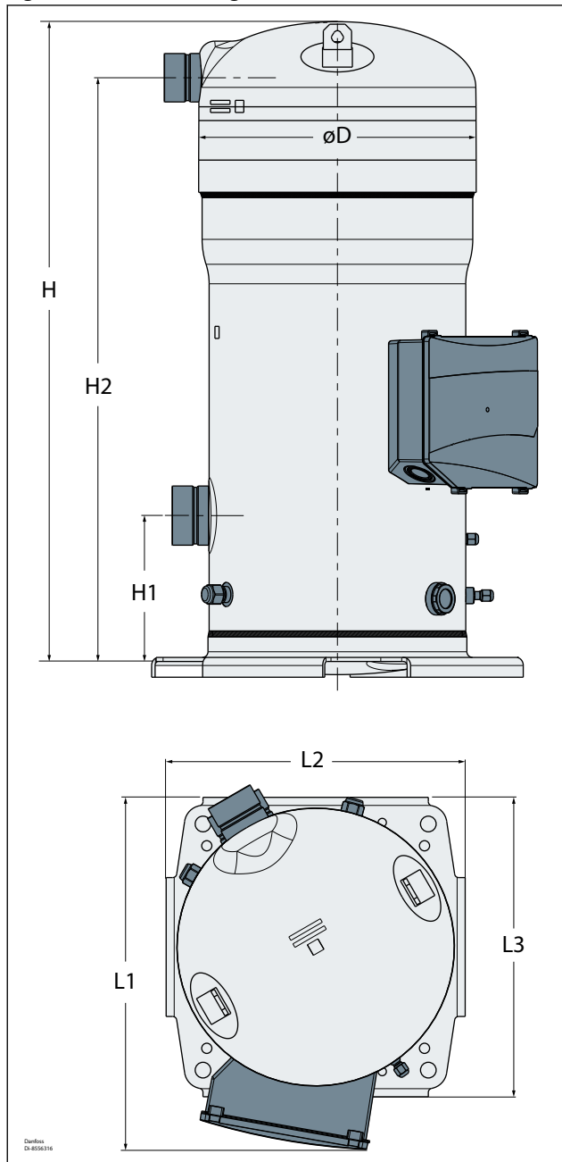
Figure 5: Outline drawing 2
