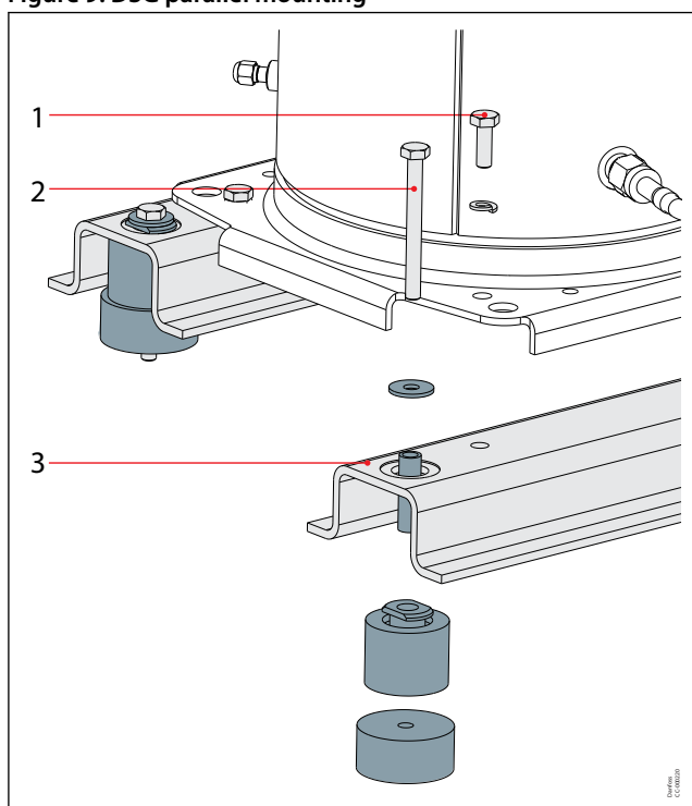
Figure 9: DSG parallel mounting
