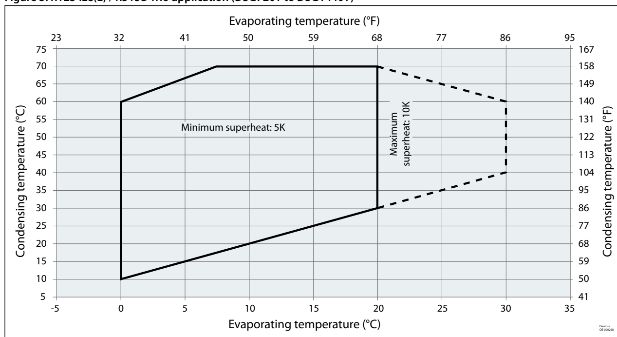
Figure 3: R1234ze(E) / R515B Trio application (DSG720T to DSG1440T)
