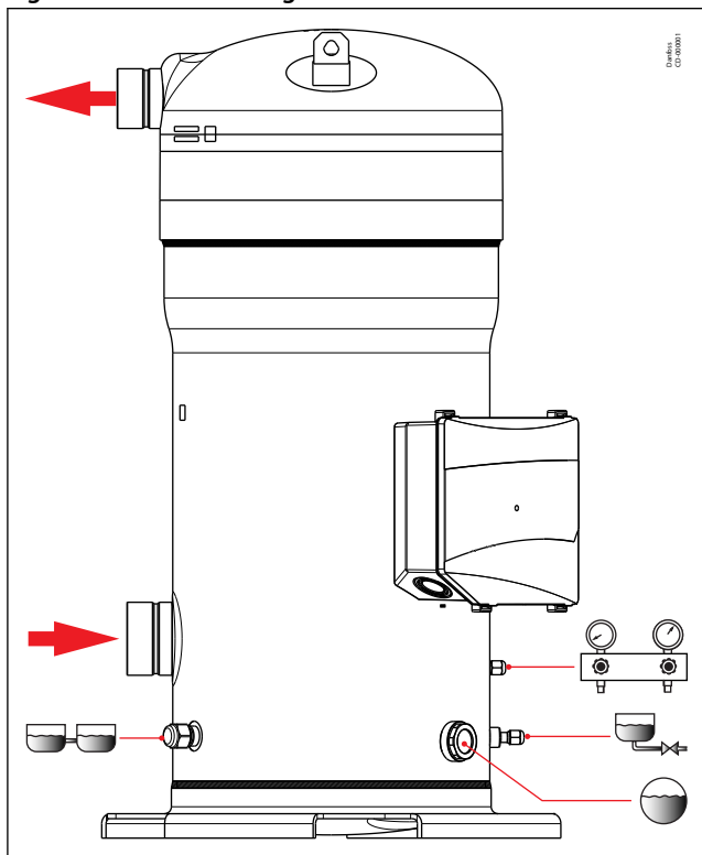
Figure 8: Outline drawing 1
