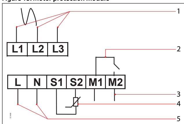
Figure 13: Motor protection module
