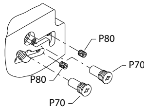
View "A" of end cap with pressure limiters, CW pump rotation. Options P
