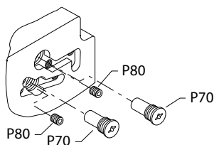
View "A" of end cap with pressure limiters, CCW pump rotation.
