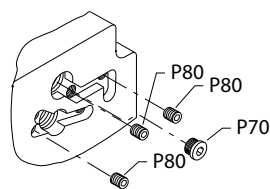
View "A" of end cap without pressure limiters, CCW and CW pump rotation.
