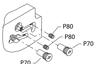
View "A" of end cap with pressure limiters, CW pump rotation.
