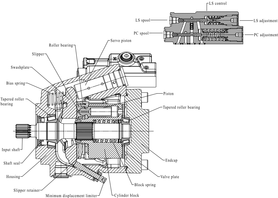
Frame X1P cross section
