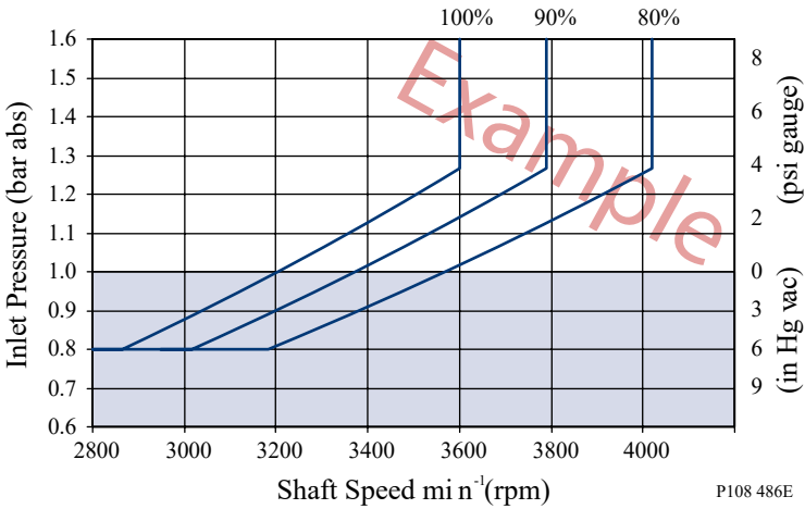
Sample inlet pressure vs. speed chart
