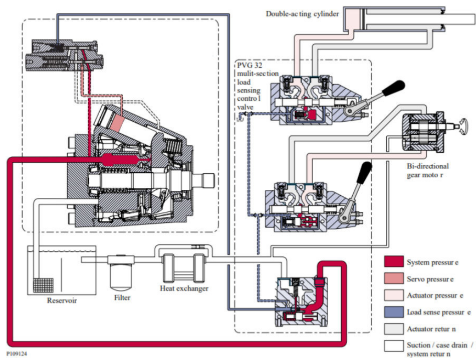
General circuit diagram
