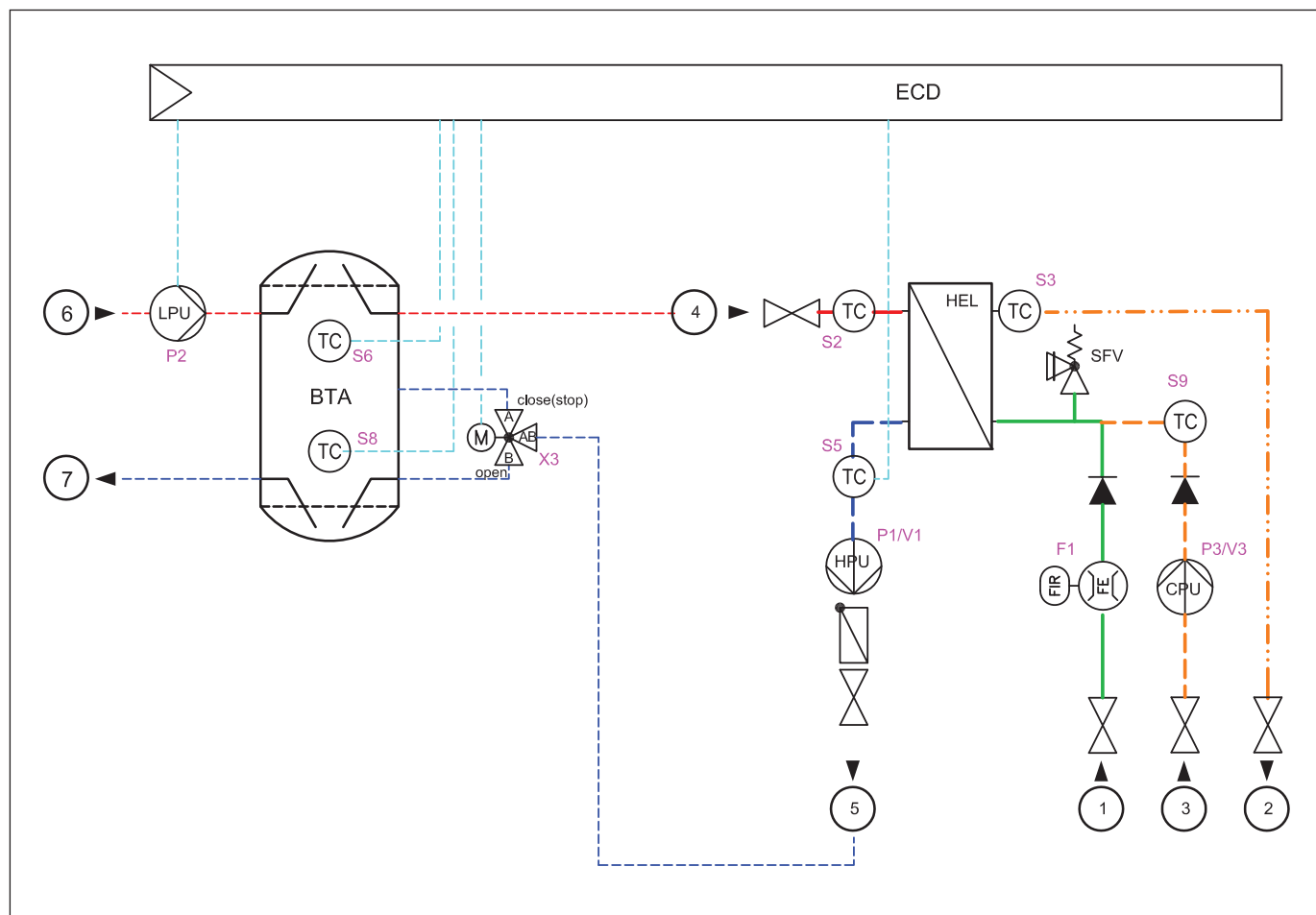
Example: stratification control and buffer tank charging with application P318.11, ex. a
