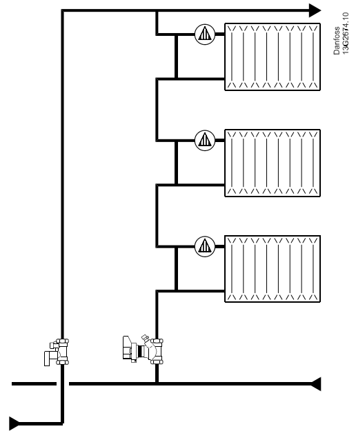
1-pipe system
