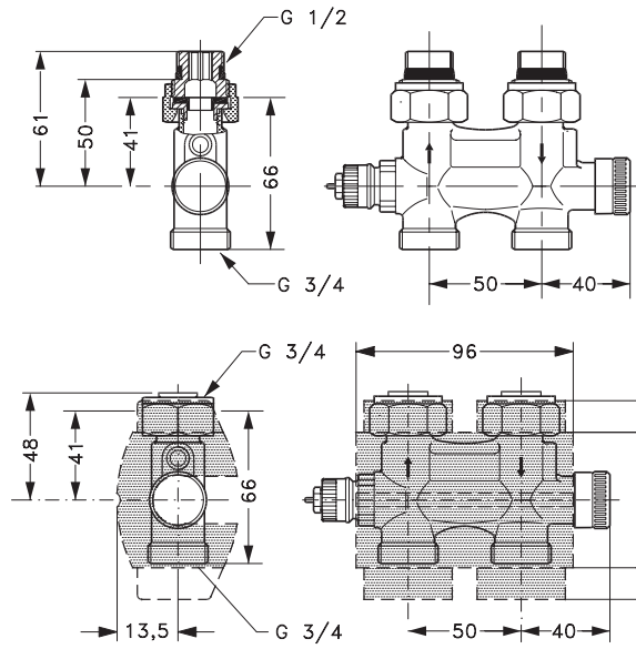
VHS straight pattern 1/2 or 3/4" radiator connection (covers are shaded grey).
