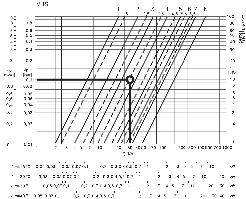
Capacities, using RA 2000 sensor elements at a P-band between 0.5 K and 2 K.
