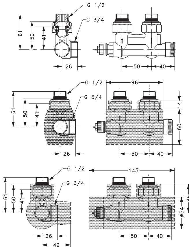
VHS angle pattern 1/2 or 3/4" radiator connection (covers are shaded grey).
