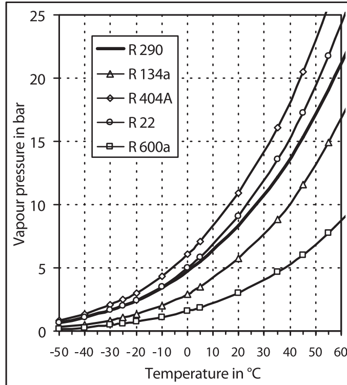
Figure 4: Vapour pressure of different refrigerants versus temperature
