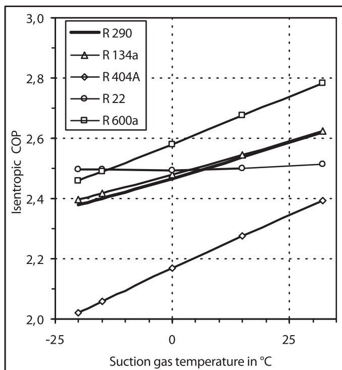
Figure 8: Theoretical COP increase of different refrigerants versus suction temperature with adiabatic compression, internal heat exchange, at -25 °C evaporation, 45 °C condensation, no subcooling before internal heat exchanger
