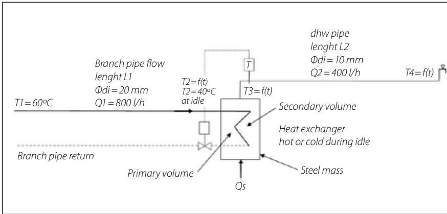
FIGURE 6: Basic application for flat station, including boundary conditions for dynamic simulations
