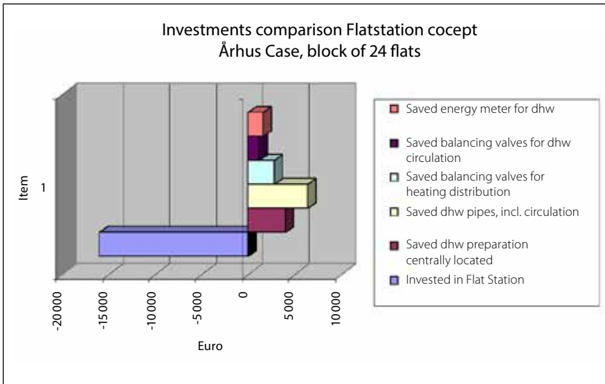
FIGURE 2: Investment balance for traditional system C and flat system F. Block of 24 flats
