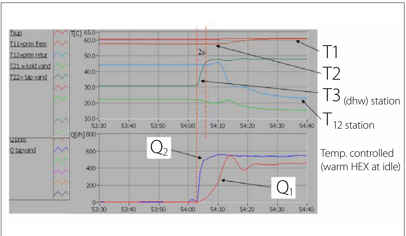
FIGURE 5: Dynamic control performance (idle recovery) for thermostatic controlled heat exchanger for dhw production. Heat exchanger is warm during idle. [7]
