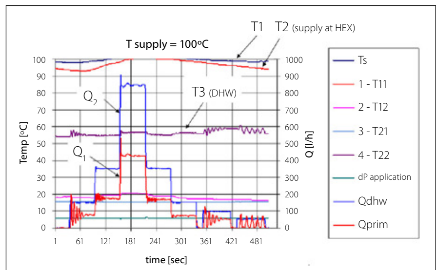
FIGURE 3: Dynamic control performance (step test) for thermostatic and pressure controlled heat exchanger for dhw production [6]
