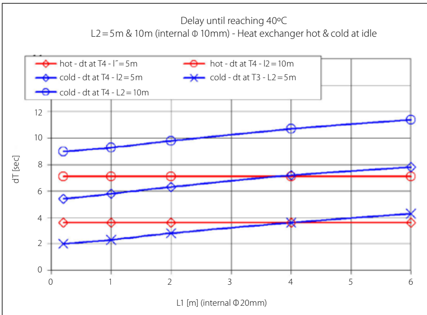
FIGURE 7: Dynamic simulation results for hot and cold heat exchanger during idle. Delay (dt) for dhw temp. of 40°C
