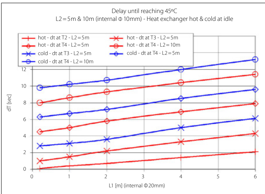
FIGURE 8: Dynamic simulation for hot and cold heat exchanger during idle. Delay (dt) for dhw temp. of 45°C
