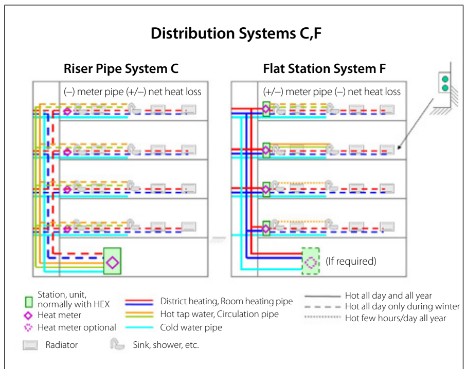
FIGURE 1: Pipe distribution systems in blocks of flats. C: Modern reference principle. F: Flat station principle
