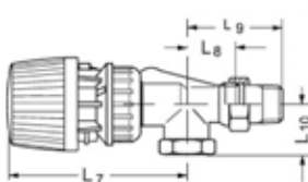
Horizontal Angle RA-FN 10, 15, 20 & RA-FN 10 or 20
