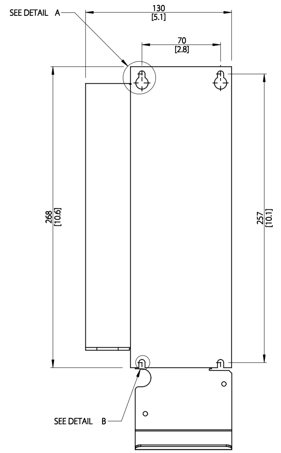
MOUNTING BASE
