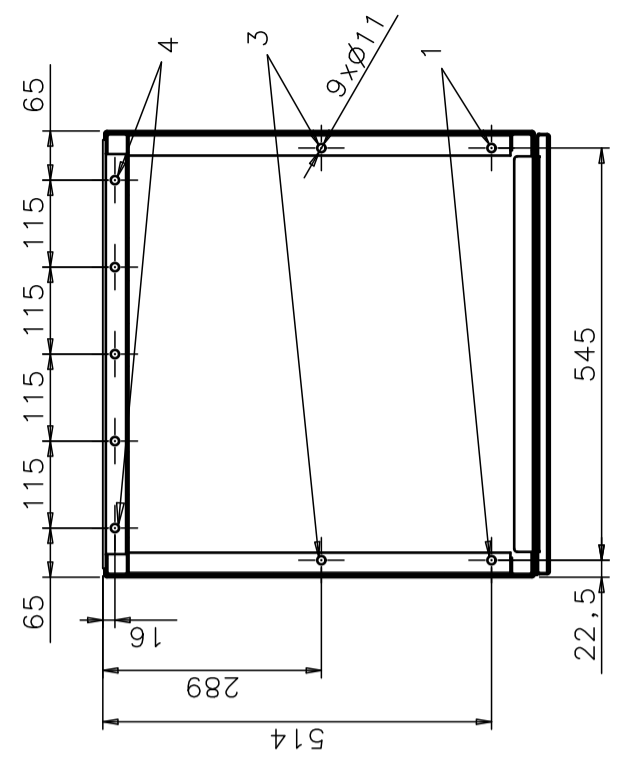
Section A-A, Floor fixation
