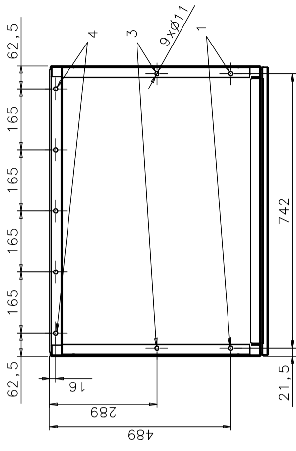
Section A-A, Floor fixation
