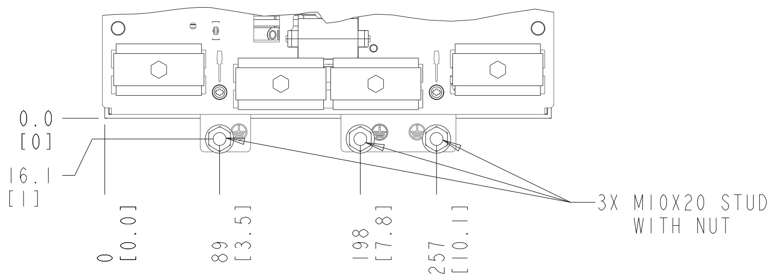
MOTOR TERMINAL
