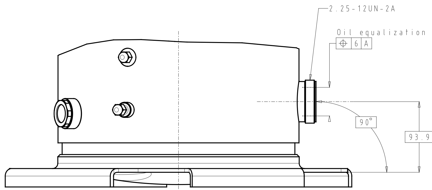
VIEW H
