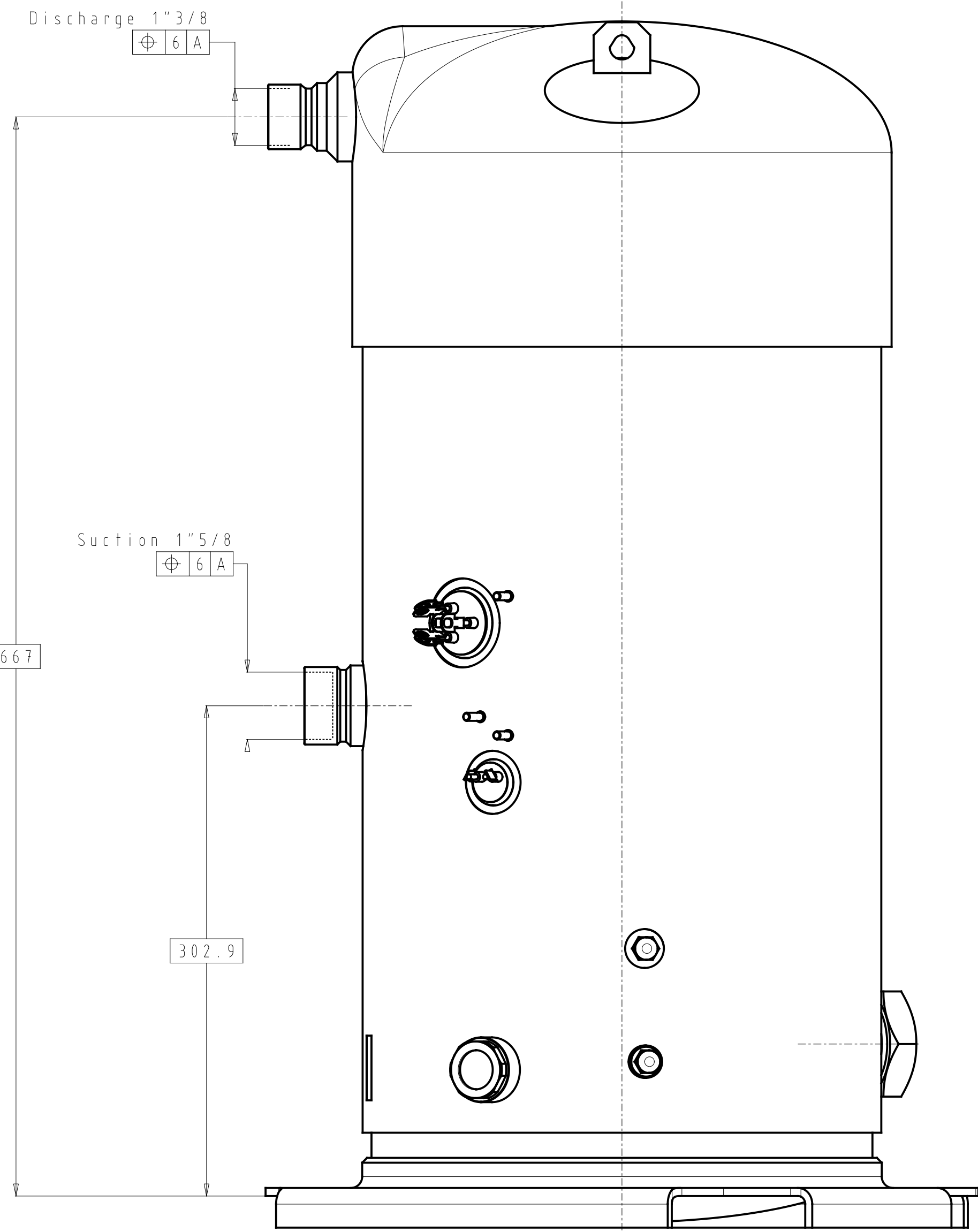
VIEW J
