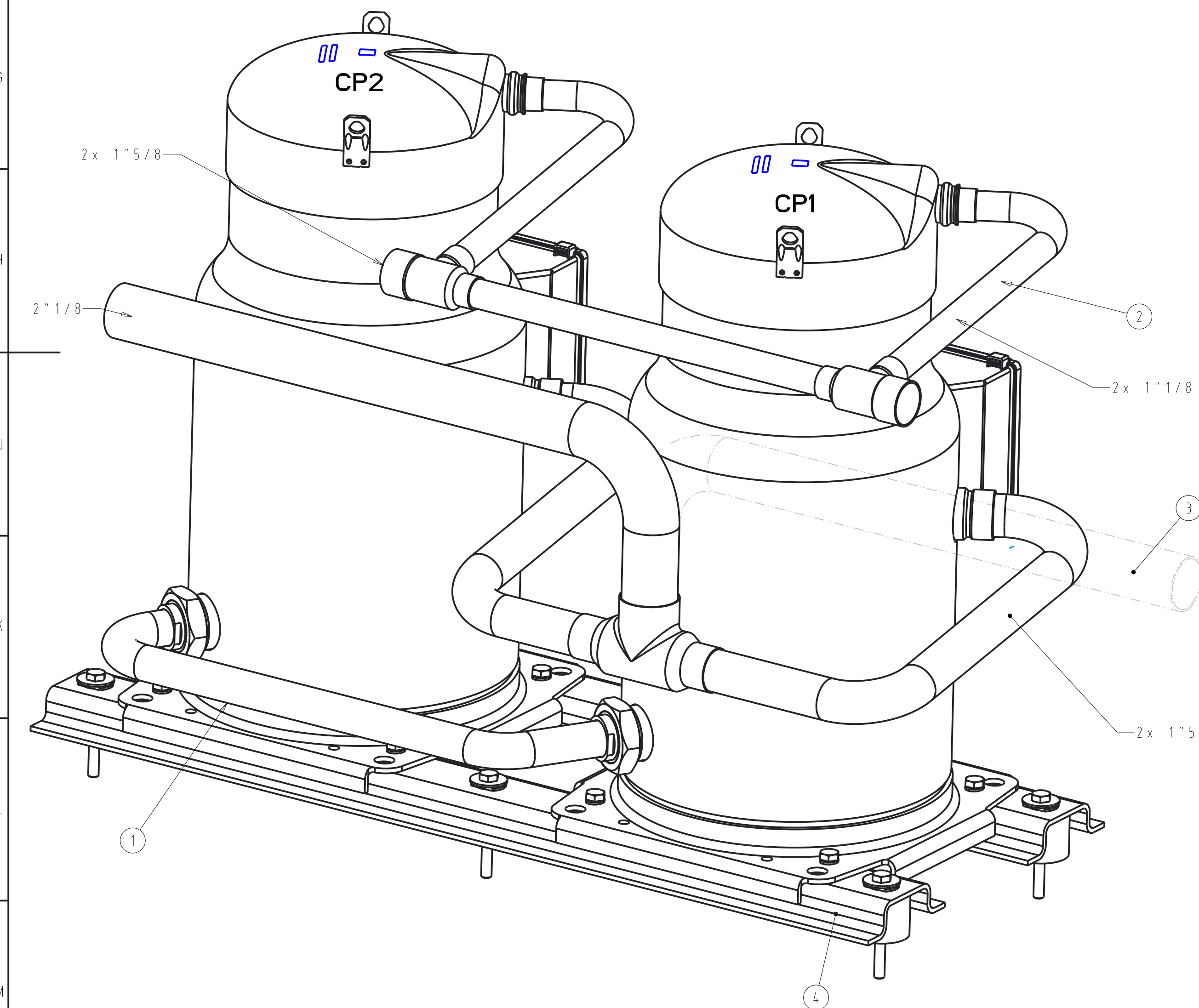
MANIFOLDING MOUNTING KIT 120Z0792 120Z0795 120Z0796 SCALE 1/1
