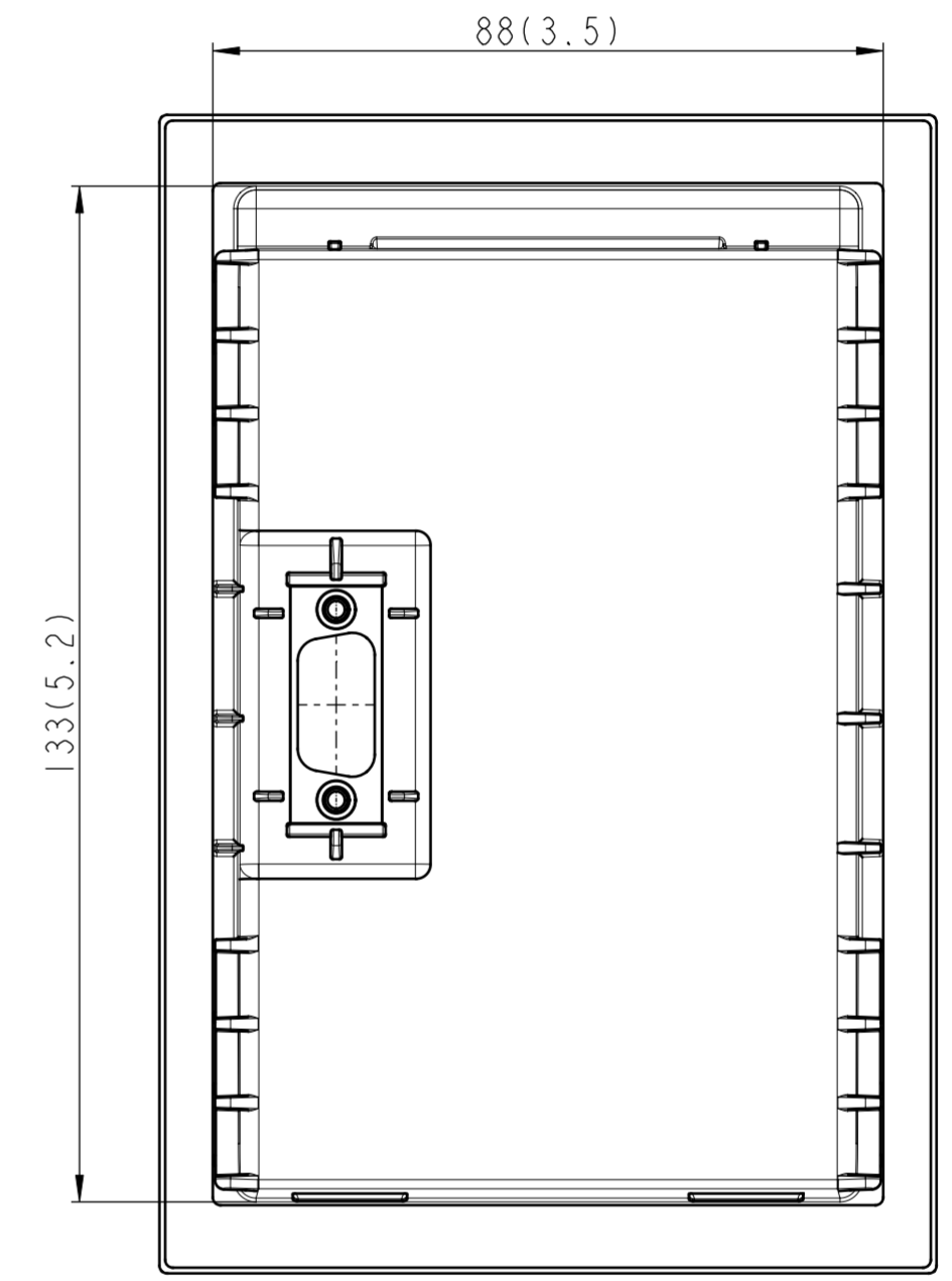
Flush Mounting Drilling dimension View from front in mm(in)
