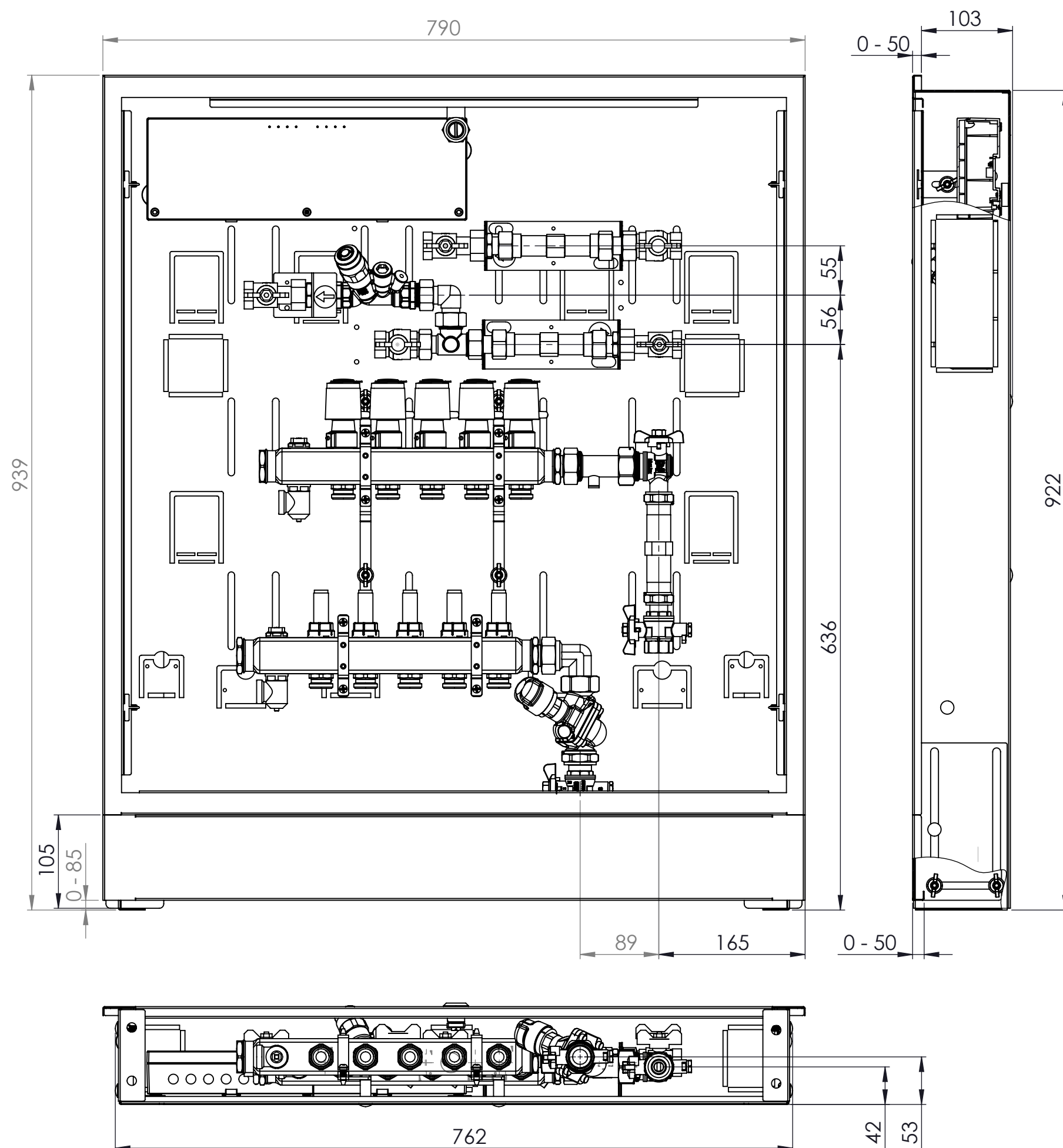
088X4115 UnoFloor Metering Comfort right 5-loops
