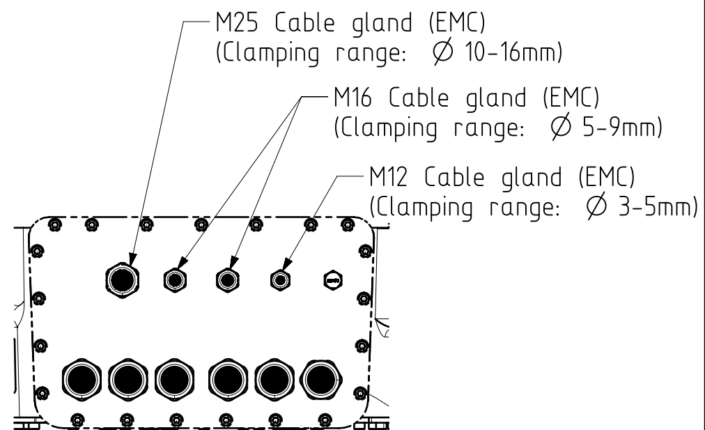
SECTION C-C Low voltage connections, N-END (+LVB1, optional)
