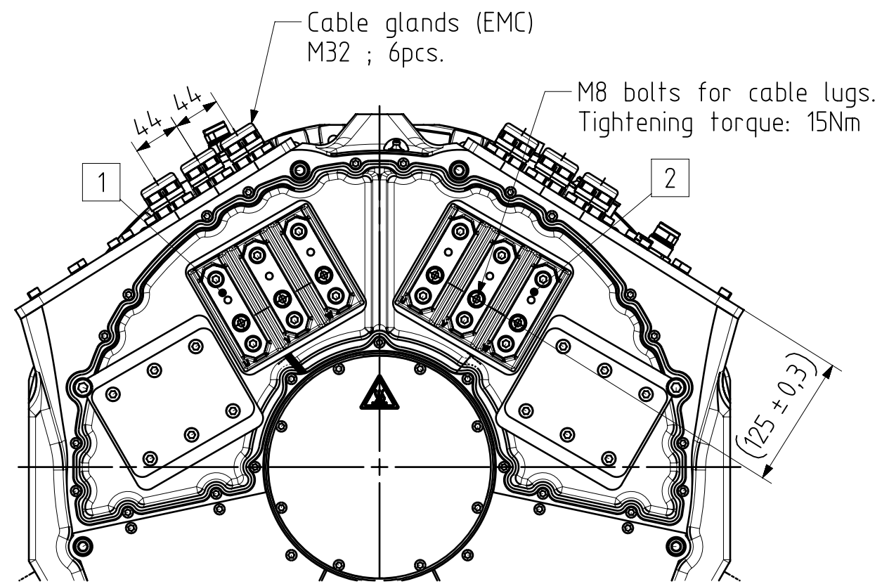
Terminal box, DUAL DUAL winding systems 1-2 marked with squares □
