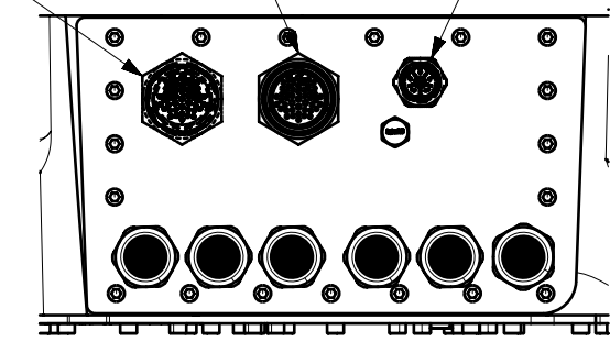
SECTION B-B Low voltage connectors, N-END
