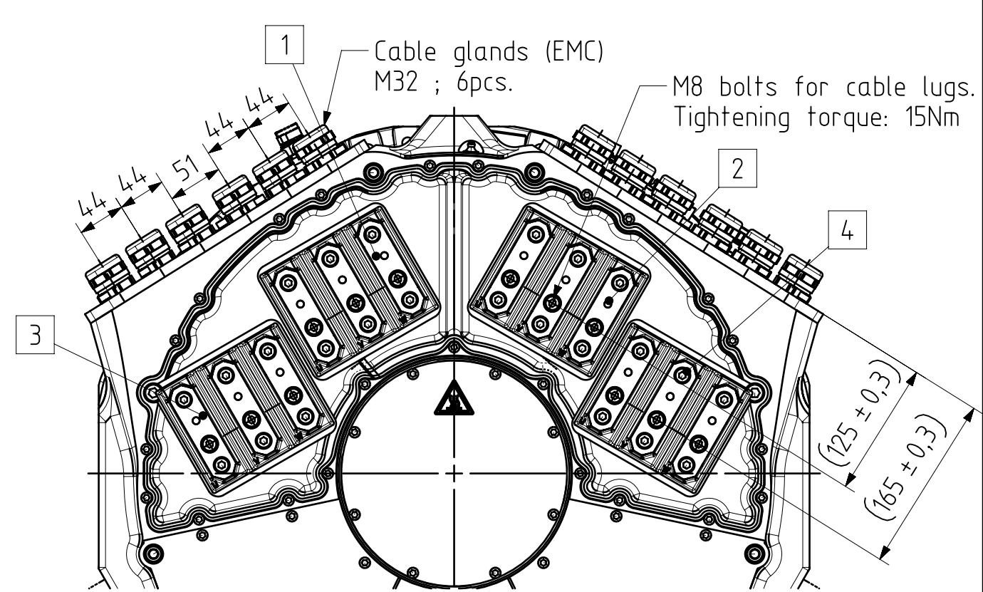
Terminal box, QUAD QUAD winding systems 1-4 marked with squares □
